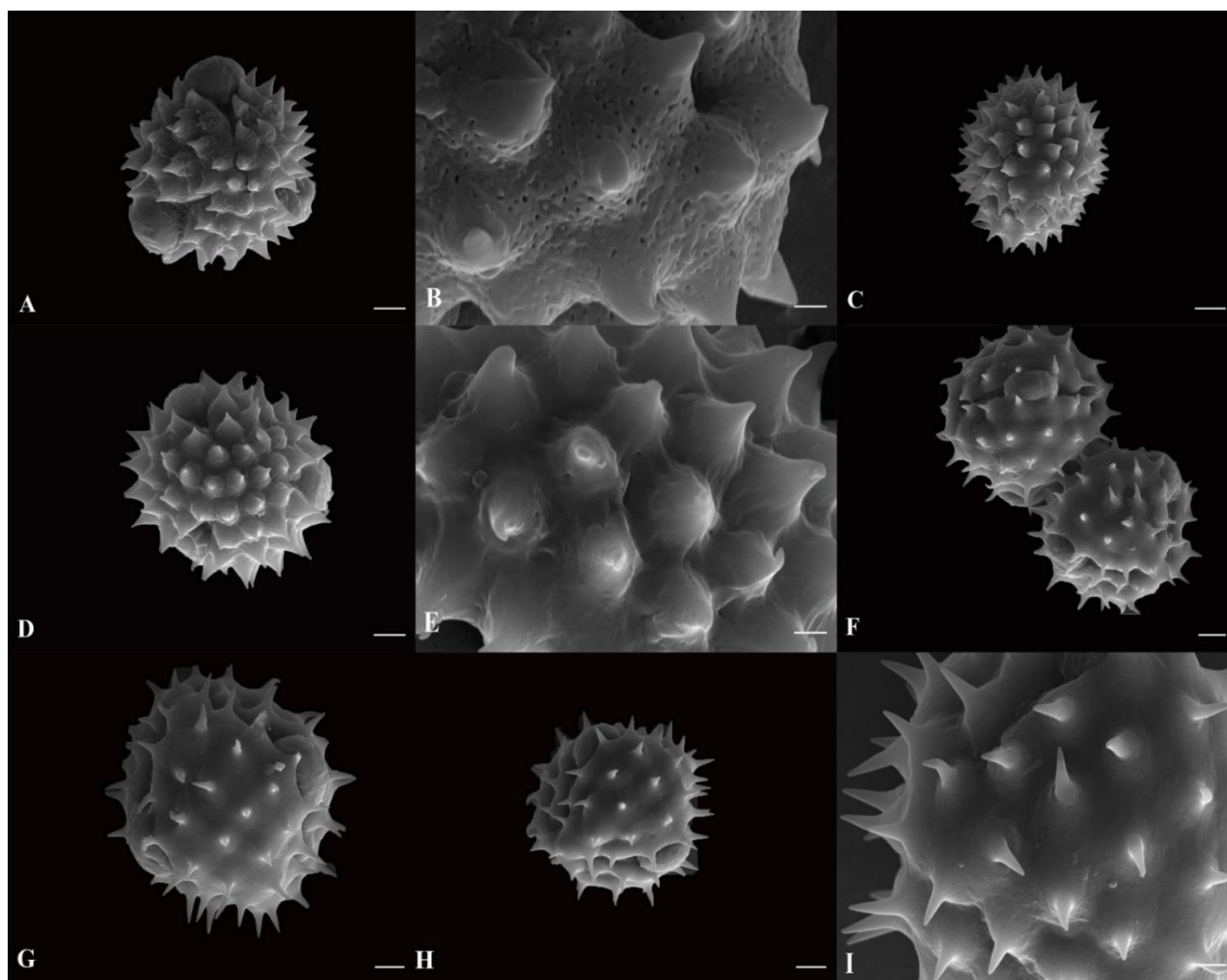
Fig. 3. SEM micrographs of pollen grains in the studied species of Gnaphalieae and Calenduleae: A. Phagnalon persicum , polar view, B. Phagnalon persicum , exine sculpture, C. Pseudognaphalium luteoalbum , equatorial view, D. Pseudognaphalium luteoalbum , polar view, E. Pseudognaphalium luteoalbum , exine sculpture, F. Calendula officinalis , overview of two grains, G. Calendula officinalis , equatorial view, H. Calendula officinalis , polar view, I. Calendula officinalis , exine sculpture (Bars: F, G, H = 10 µm, A, C, D, I = 2 µm, B, E = 1 µm).
