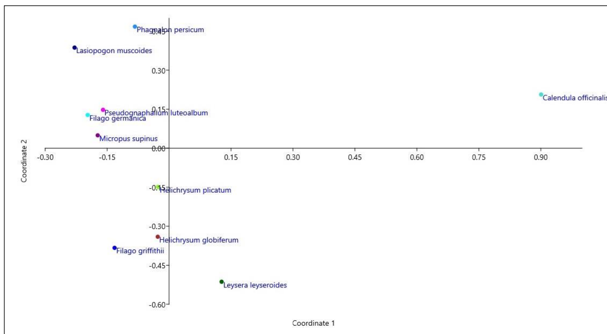
Fig. 6. PCoA plot of the studied species of Gnaphalieae and Calenduleae based on pollen data (species according to Appendix 1).
